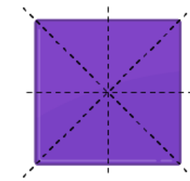
Square 4 Lines of symmetry
