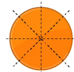
Circle Infinite Lines of symmetry
