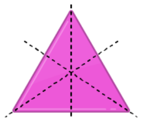
Equilateral Triangle 3 Lines of symmetry
